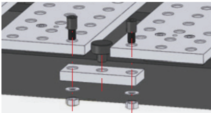
Mount the Channel Block and insert the Rest Button to create a continuous work surface over the table slot.
